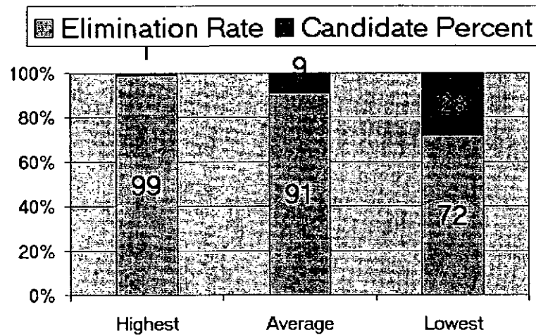
Fig. 4-16. The performance of the global feature based selection scheme: elimination rate vs. candidate percentage
