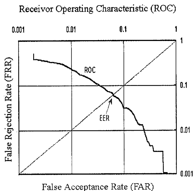
Fig. 2-1 ROC curve
