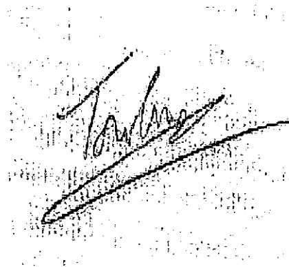
Fig. 1-4 Signature sample
