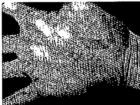
Fig. 1-2 Palmprint sample
