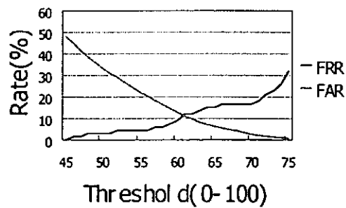
Fig. 5-24 Relationship of FRR, FAR and Threshold of Matching Crucial Set to Whole Feature Set
