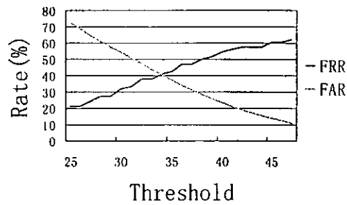
Fig. 5-23 Relationship of FRR, FAR and Threshold of Whole Feature Set matching
