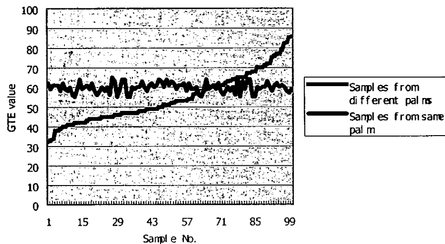
Fig. 4-13 The comparison of palmprint GTE distribution: inter-palm dispersion vs. intra-palm convergence
