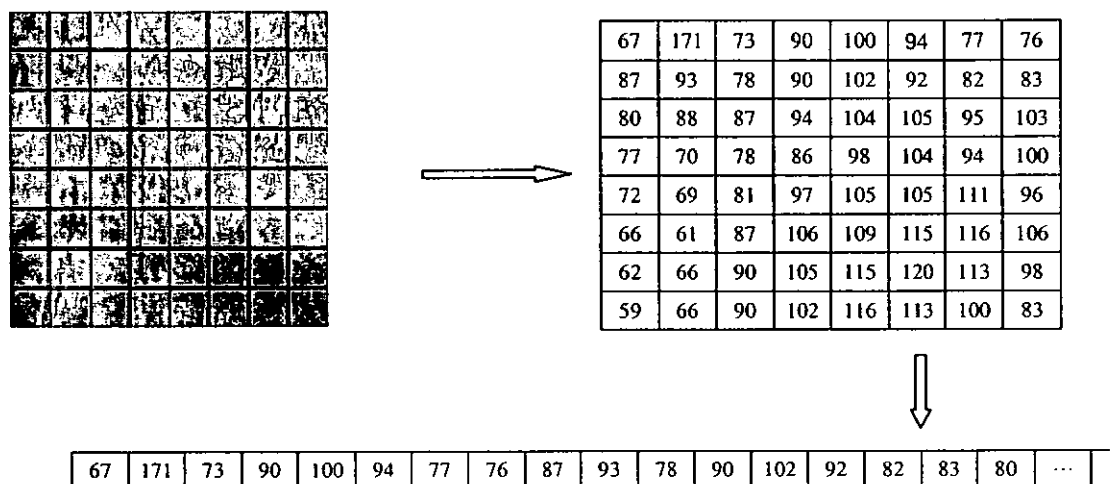
Fig. 5-12 The process of local feature extraction.
