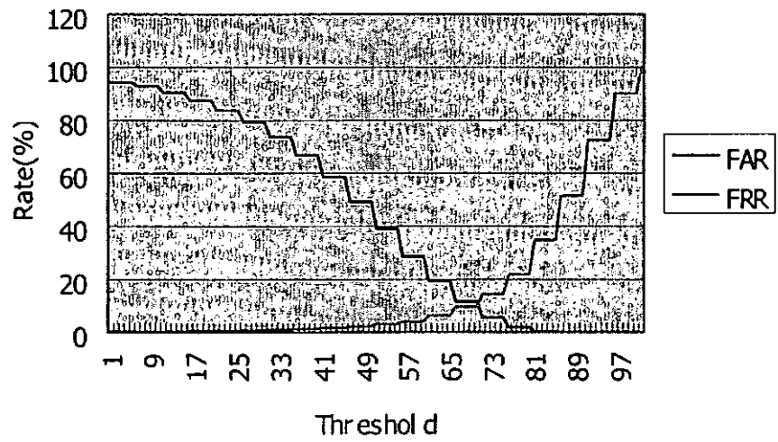
Fig. 6-4 FAR and FRR of Fourier Transform
