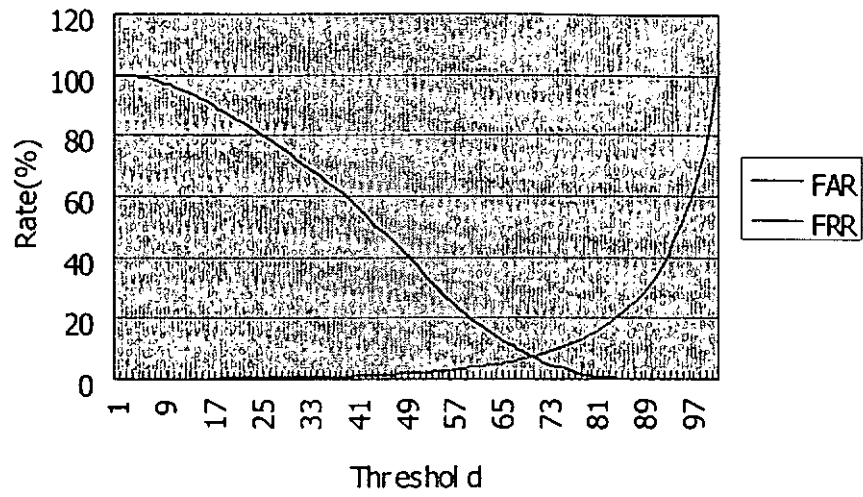
Fig. 6-3 FAR and FRR of texture analysis
