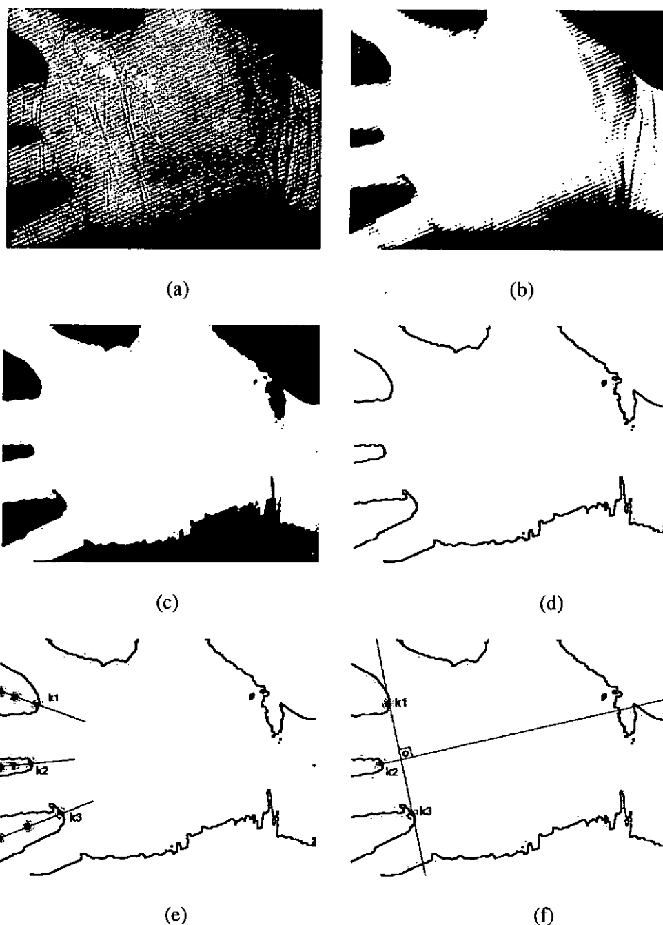
Fig. 5-3 Determination of K1, K2 and k3 (a) the original image (b) the binary map of the original image (c) smoothed map of (b) (d) palmprint boundary (e) determination of K1, k2 and K3 (f) determination of the coordinate system
