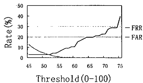
Fig. 5-25 Relationship of FRR, FAR and Threshold of Bi-directional Matching
