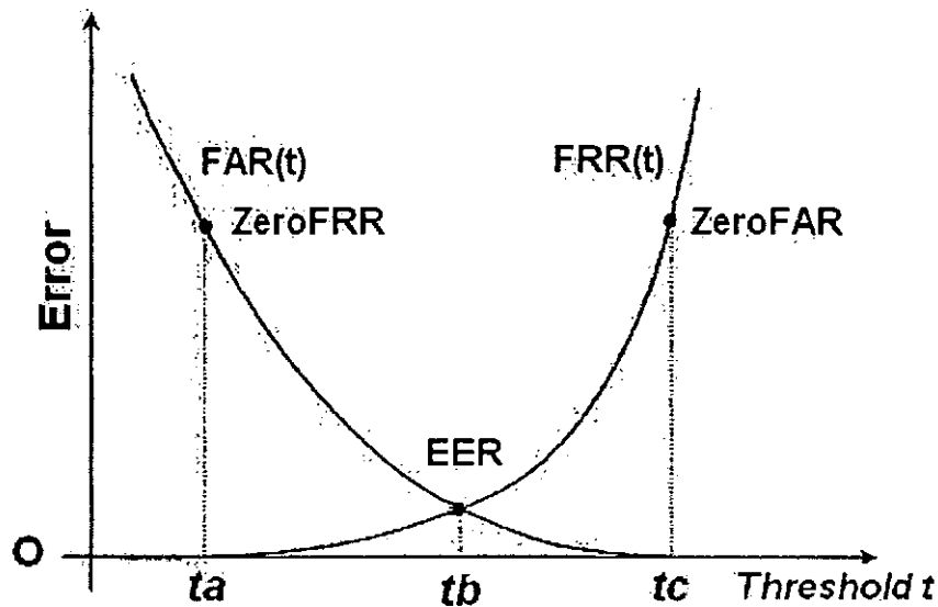
Fig. 6-2 An example of FAR/FRR curve, where the points corresponding to EER, ZeroFAR and ZeroFRR are highlighted.
